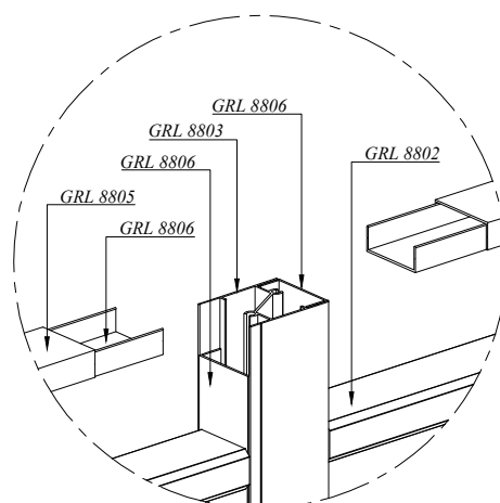
DETAILS B'
