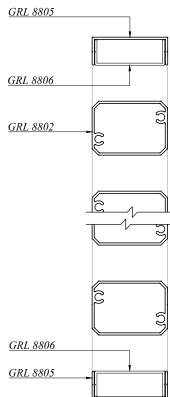
SECTION A
