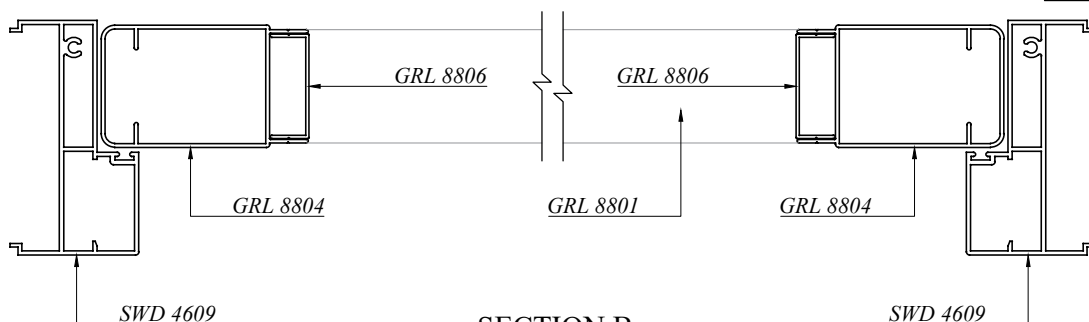
SECTION B
