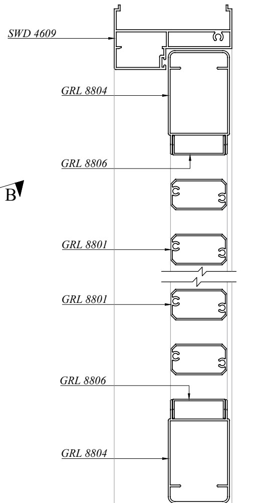
SECTION A
