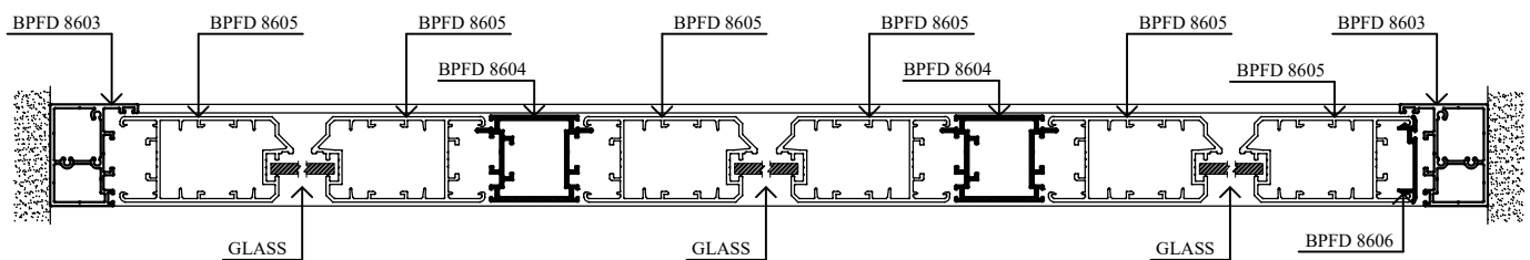
SECTION VIEW B - B
