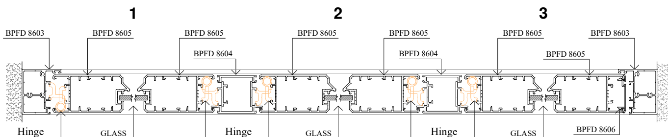
SECTION VIEW B - B
