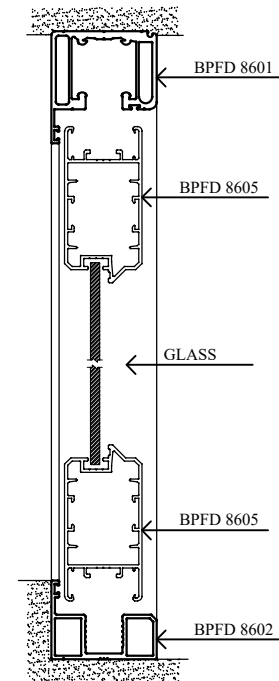
SECTION VIEW A - A
