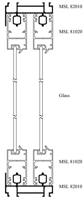
SECTION VIEW A - A
