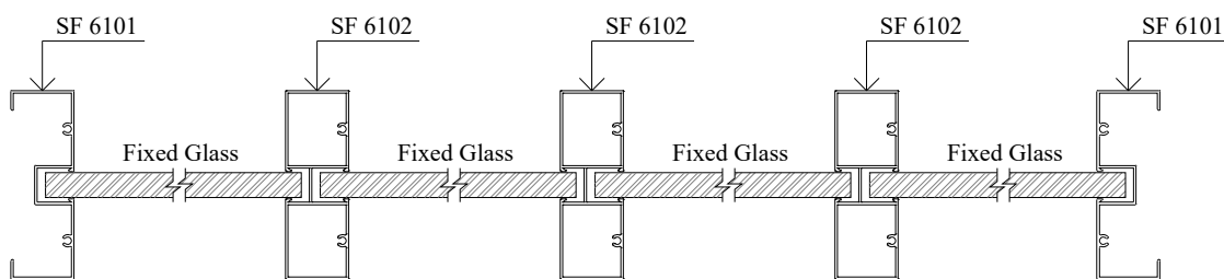
SECTION VIEW A - A
