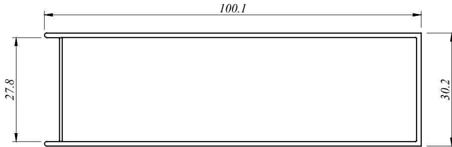
MISC 5147 0.817 Kg/M AP : 267.950 MM
