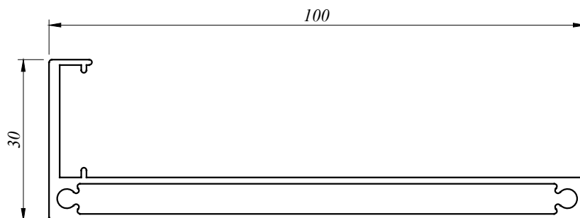
MISC 5139 0.889 Kg/M AP : 483.310 MM
