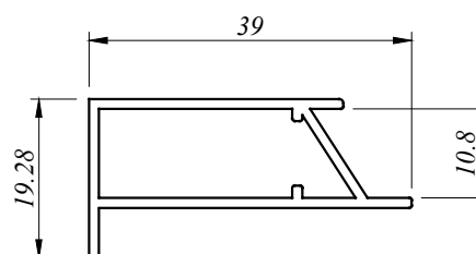
MISC 5108 H 0.342 Kg/M AP : 118.840 MM
