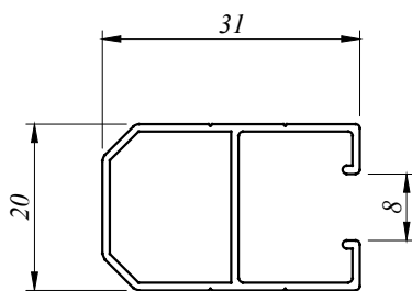
MISC 5116 0.261 Kg/M AP : 149.715 MM
