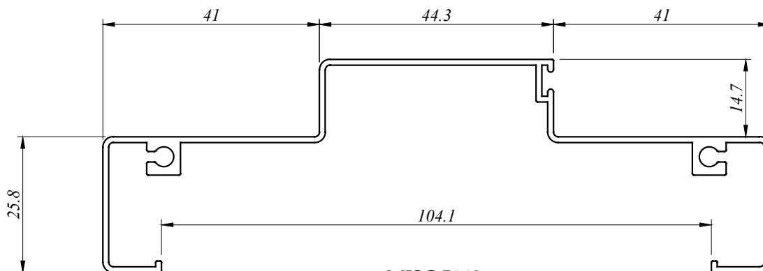
MISC 5148 0.842 Kg/M AP : 501.381 MM
