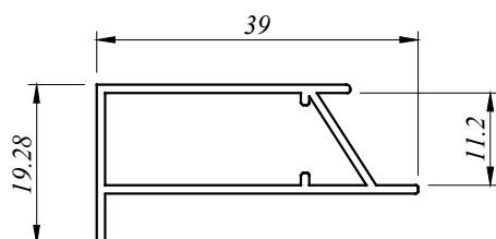
MISC 5108 0.306 Kg/M AP : 118.659 MM
