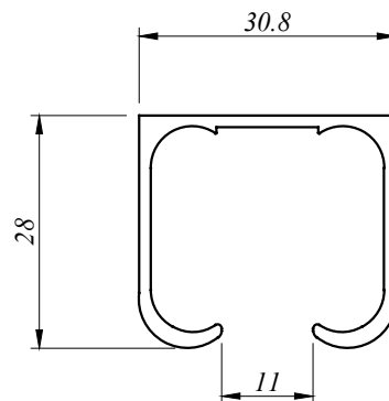
MISC 5148 0.842 Kg/M AP : 501.381 MM
