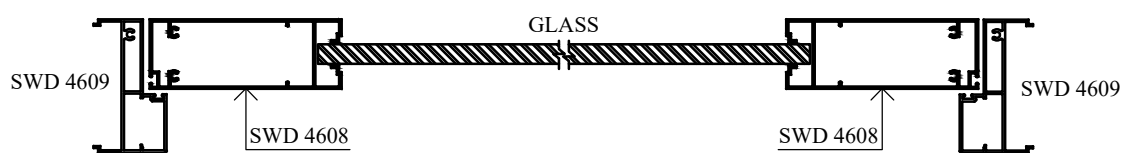
SECTION VIEW B - B
