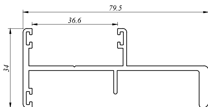
SD 4403 0.945 Kg/M AP : 340.845 MM
