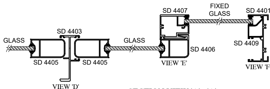
SECTION VIEW 'A' - 'A'
