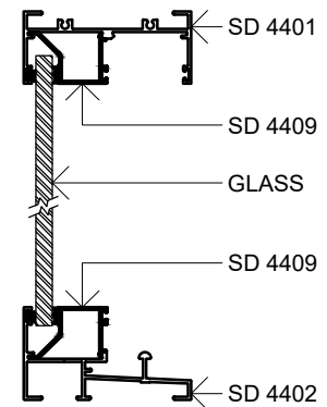
SECTION VIEW 'B' - 'B'
