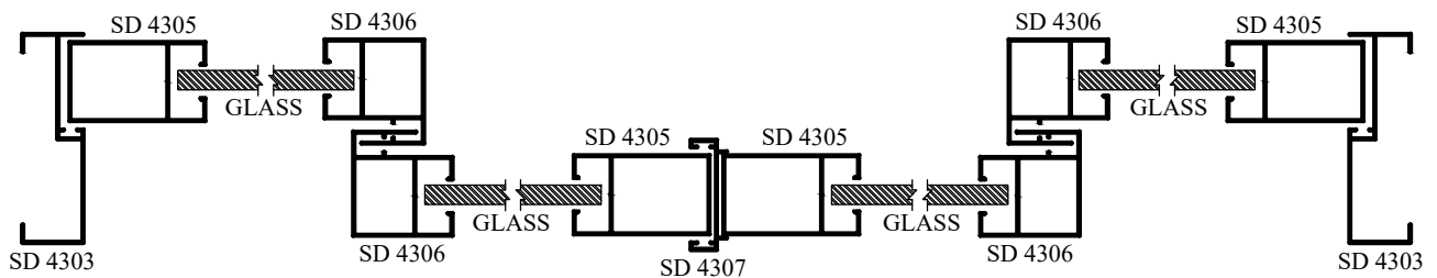
SECTION VIEW 'A' - 'A'
