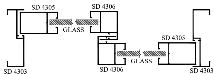
SECTION VIEW 'C' - 'C'
