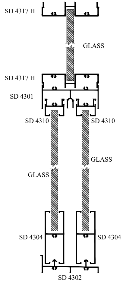
SECTION VIEW 'A' - 'A'
