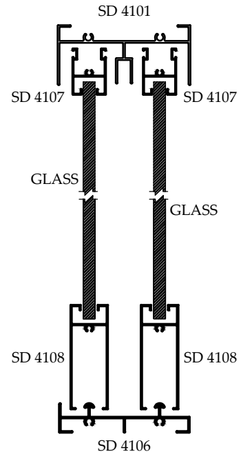
SECTION B - B
