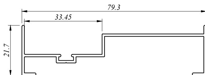
SD 4102 0.473 Kg/M AP : 291.760 MM
