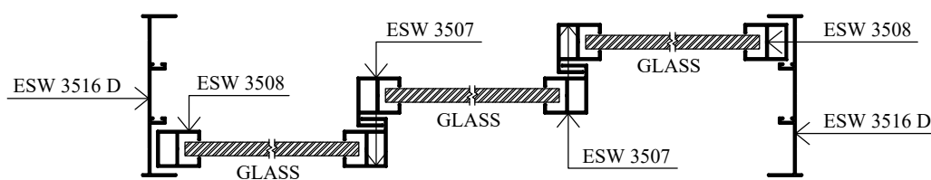
SECTION VIEW C - C
