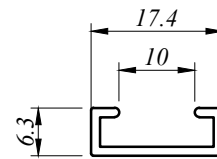
SHC 2203 0.125 Kg/M AP : 66.055 MM
