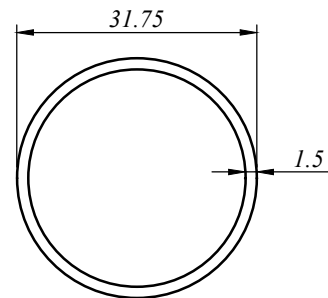
RT 141015 0.386 Kg/M AP : 99.746 MM
