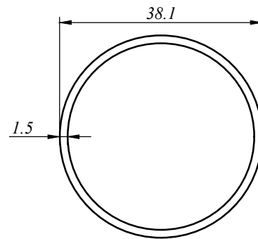
RT 141215 0.467 Kg/M AP : 119.695 MM
