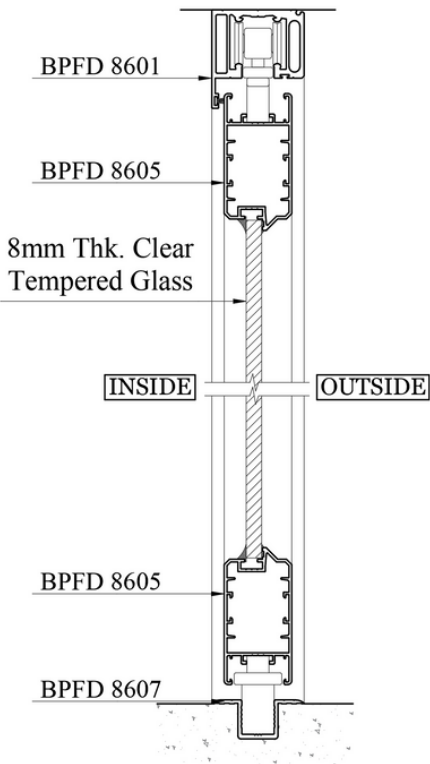
Section A
