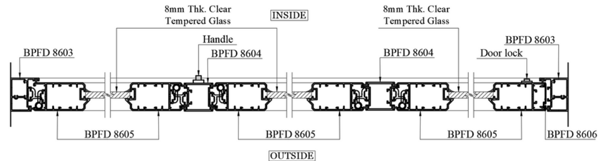
FOLDING DOOR
