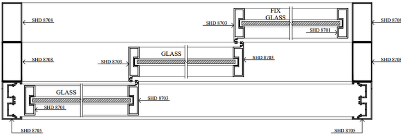
Section B
