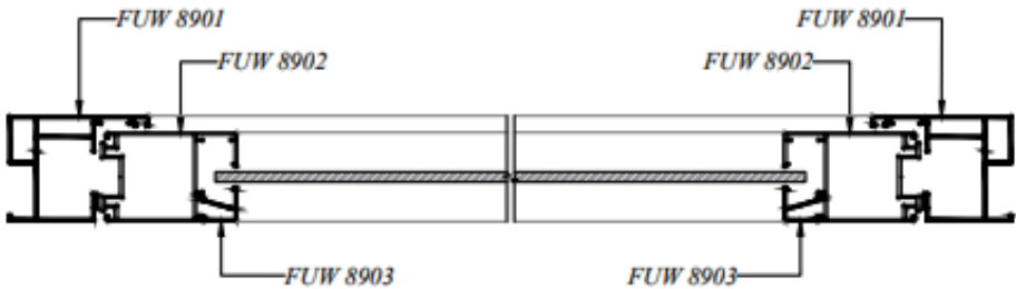
SECTION A
