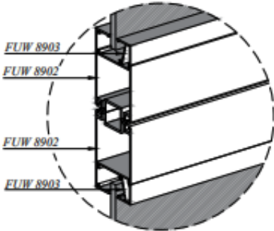
DETAILS B
