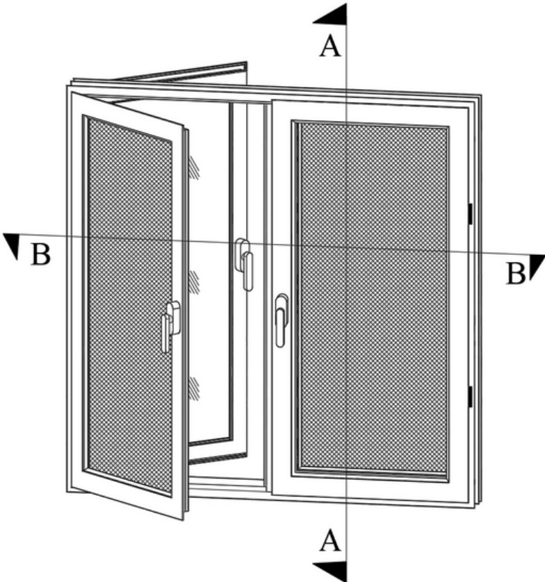
M Casement Window
