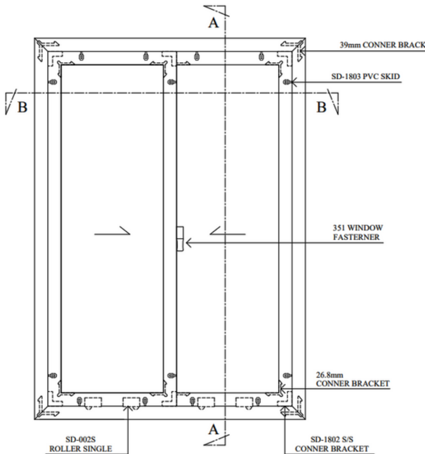
M SLIDNG WINDOW
