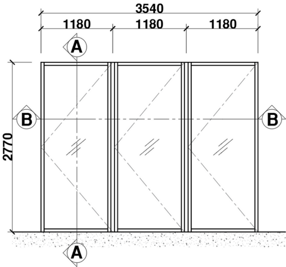
FOLDING DOOR
