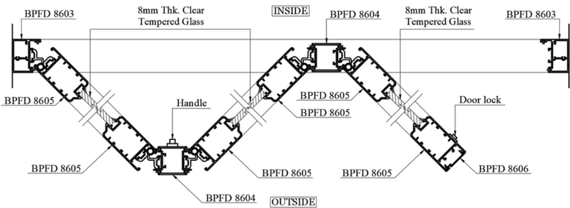
Section B
