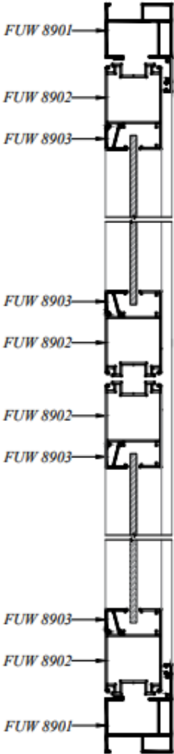
SECTION B
