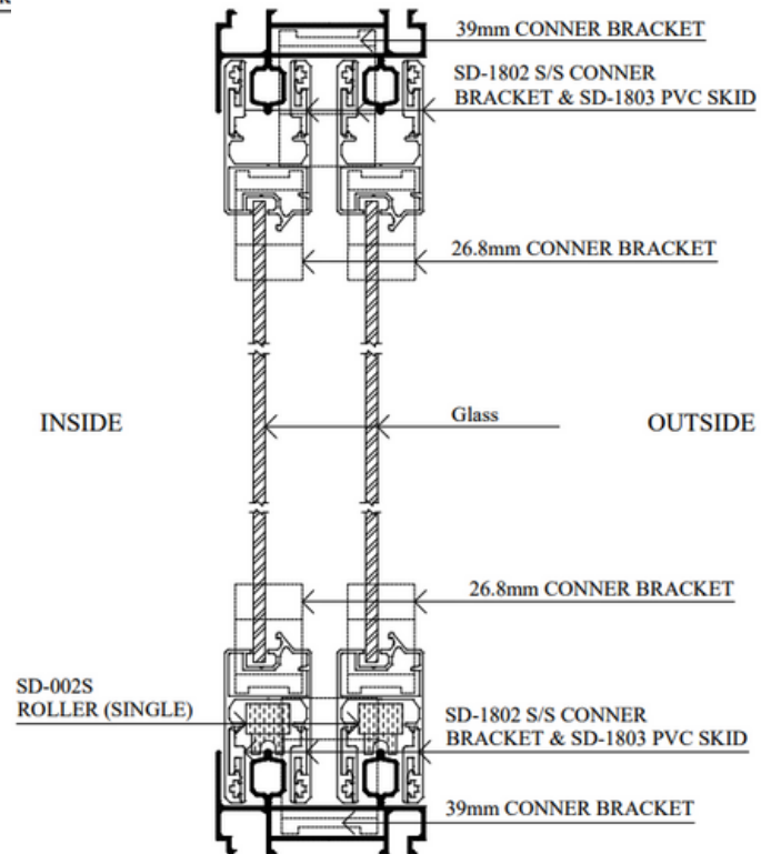
Section A
