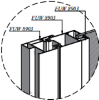
DETAILS A
