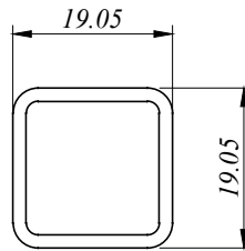
SH 25060616 0.300 Kg/M AP : 71.050 MM
